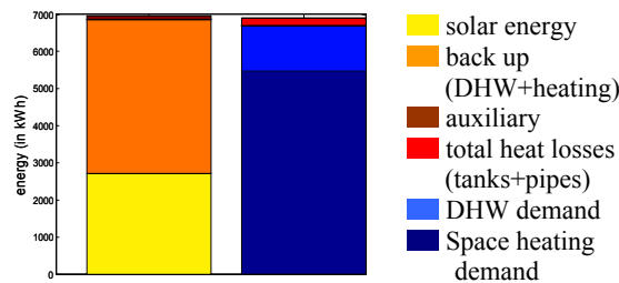
Fig. 6 Annual energy balance – Zurich (20m 2 sol. coll., 1200l storage tanks)
