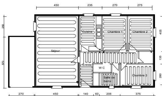
Fig. 1 Floor plan - simulation case study
