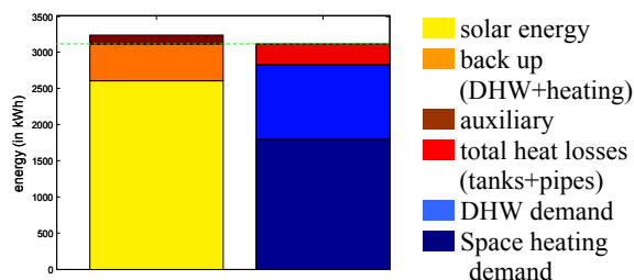
Fig. 5 Annual energy balance – Nice (15m 2 sol. coll., 900l tank)
